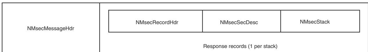
Figure 18. NMsec_GET_STACKINFO response format
