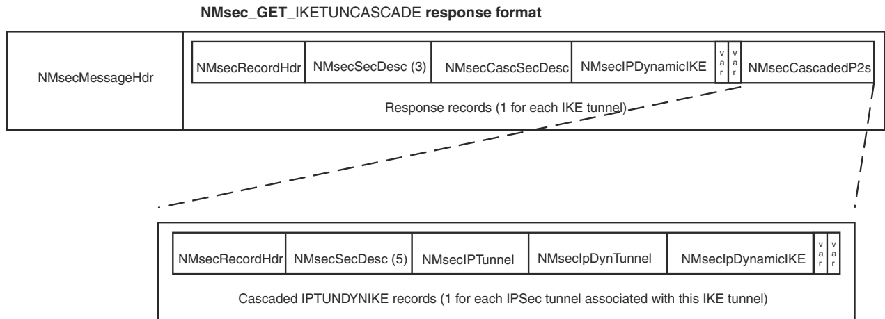
Figure 26. NMsec_GET_IKETUNCASCADE response format
