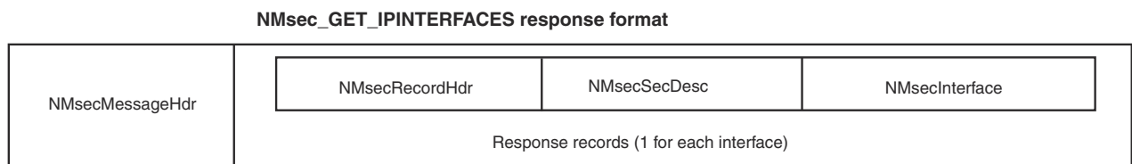
Figure 27. NMsec_GET_IPINTERFACES response format
