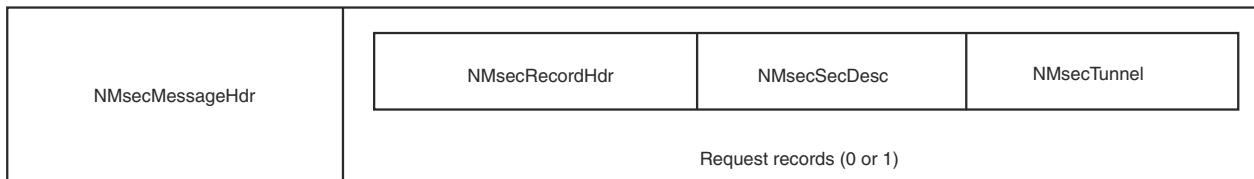
Figure 14. NMsec_DEACTIVATE_IPTUNDYN request format
